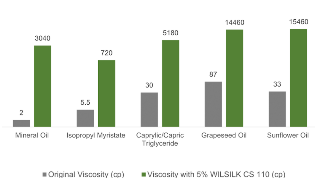
Oil Viscosity with 5% of WILSILK CS-110
